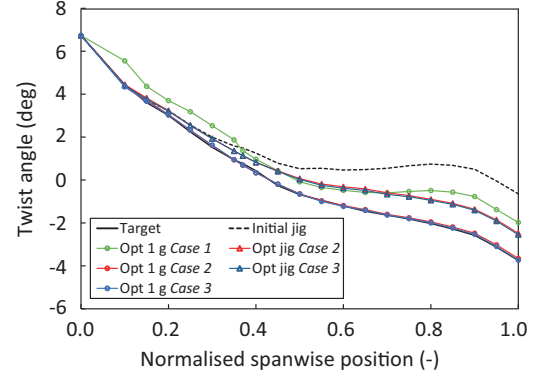
Figure 3. Cruise and jig twist distribution of the CRM wing for Cases 1, 2 and 3 .
